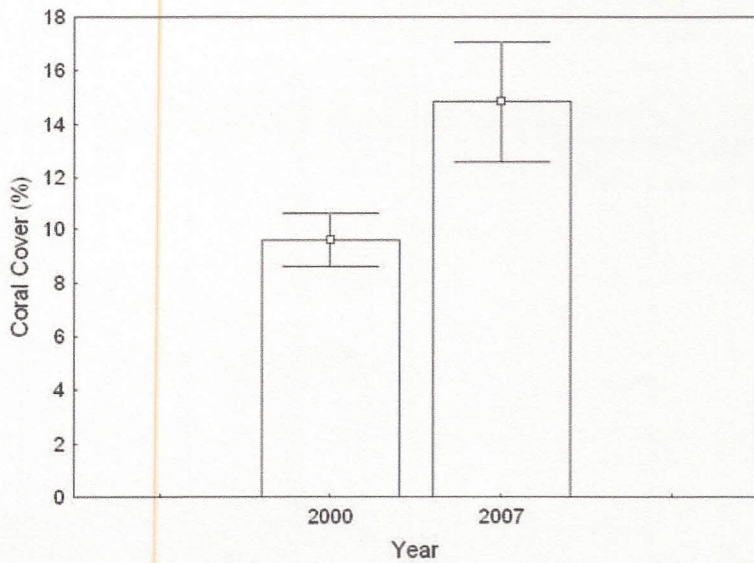
Figure 4. Coral cover at 3 m on the back reefs of Helen in 2000 and 2007; the bars show the means and the whiskers show the standard errors of the means.
